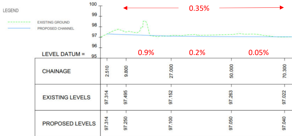
WESTERN CHANNEL – RIVER COCKER (LONG-SECTION)
