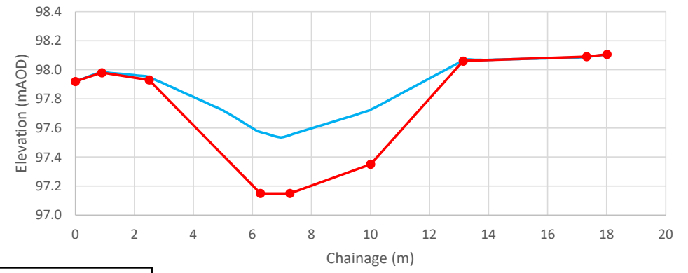
RC_06 (RIVER COCKER – EASTERN CHANNEL)
