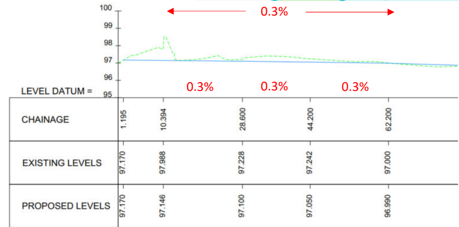
EASTERN CHANNEL – RIVER COCKER (LONG-SECTION)
