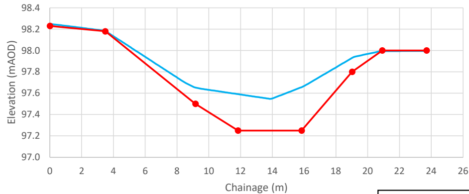
RC_01 (RIVER COCKER - WESTERN CHANNEL)
